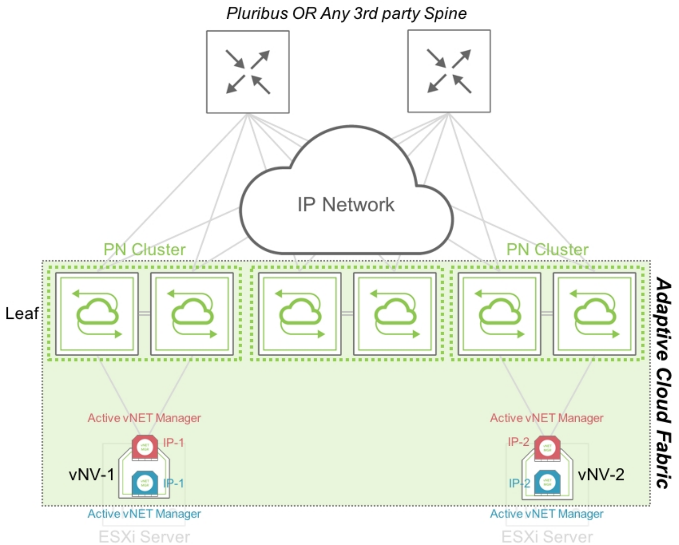
Figure 12 - vNET Manager Redundancy – Active/Active between Racks or Datacenters
