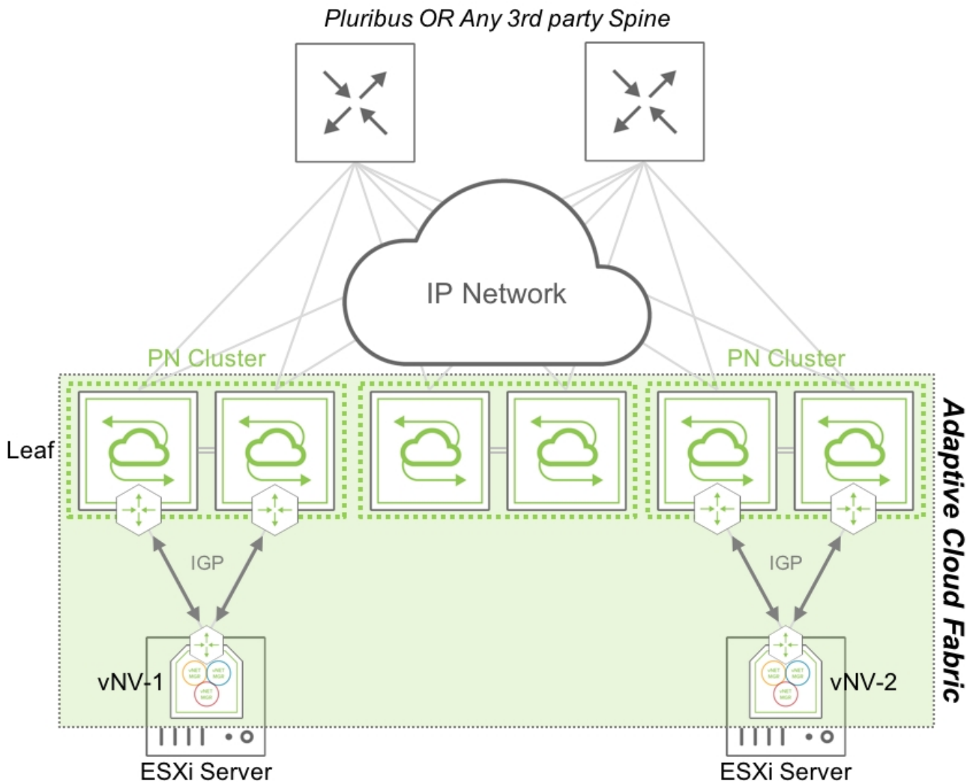
Figure 7 - Fabric Nodes in a Routed In-band Network using an IGP
