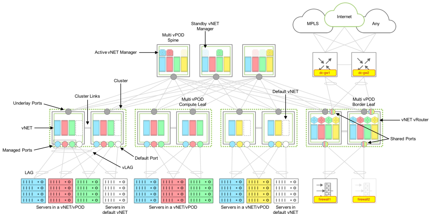
Figure 8 - Multitenant Fabric Design Components
