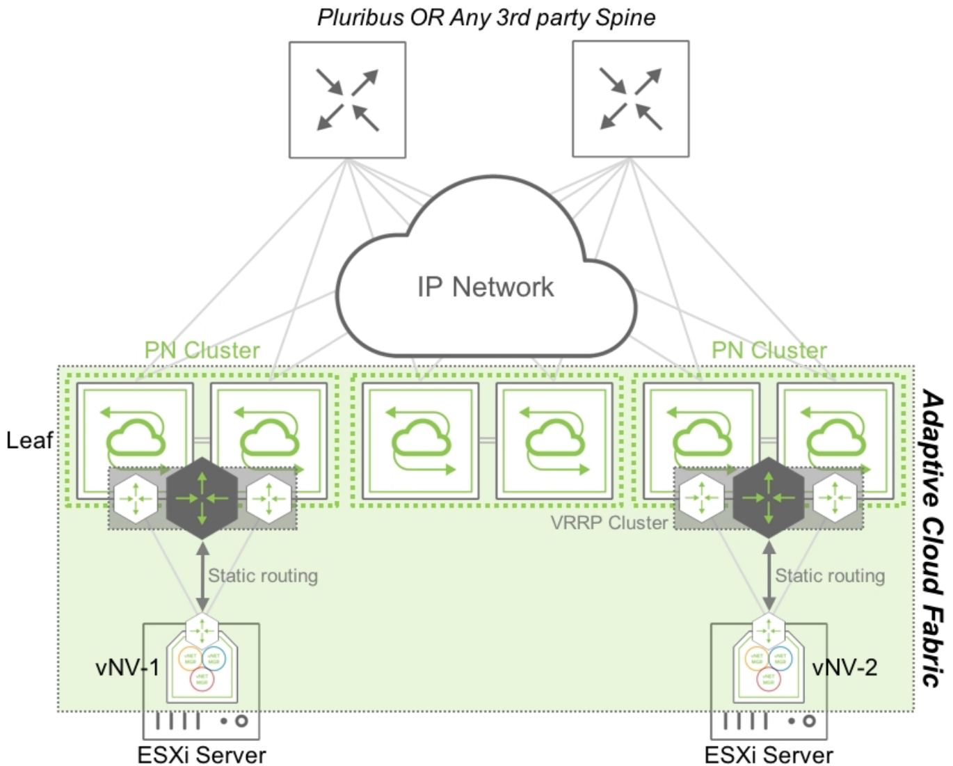
Figure 6 - Fabric Nodes in a Routed In-band Network using VRRP
