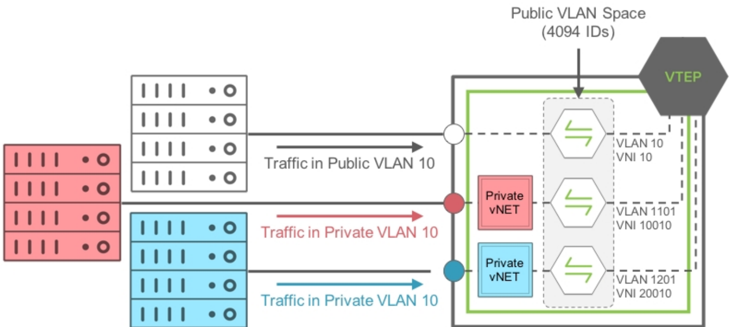
Figure 9 - Private VLAN-to-Public VLAN Mapping with Private vNETs
