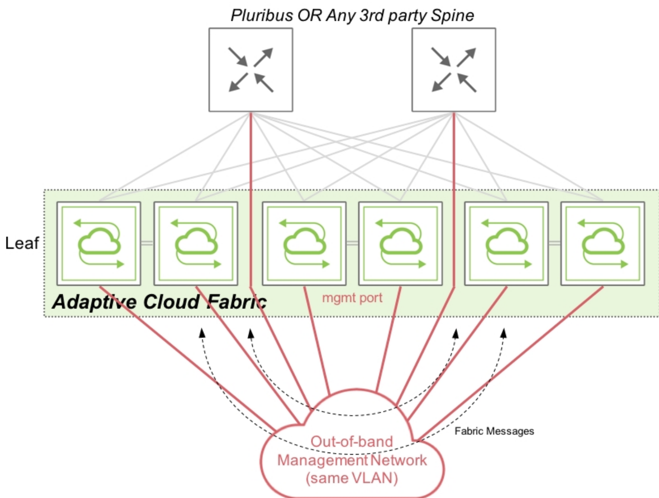
Figure 1 - Management Fabric Communications
