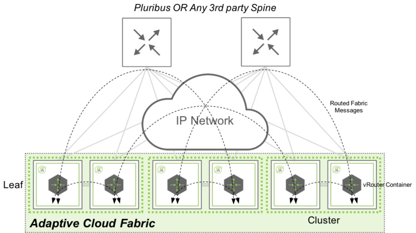
Figure 2 - In-band Fabric Communications with Layer 3 Underlay Network
