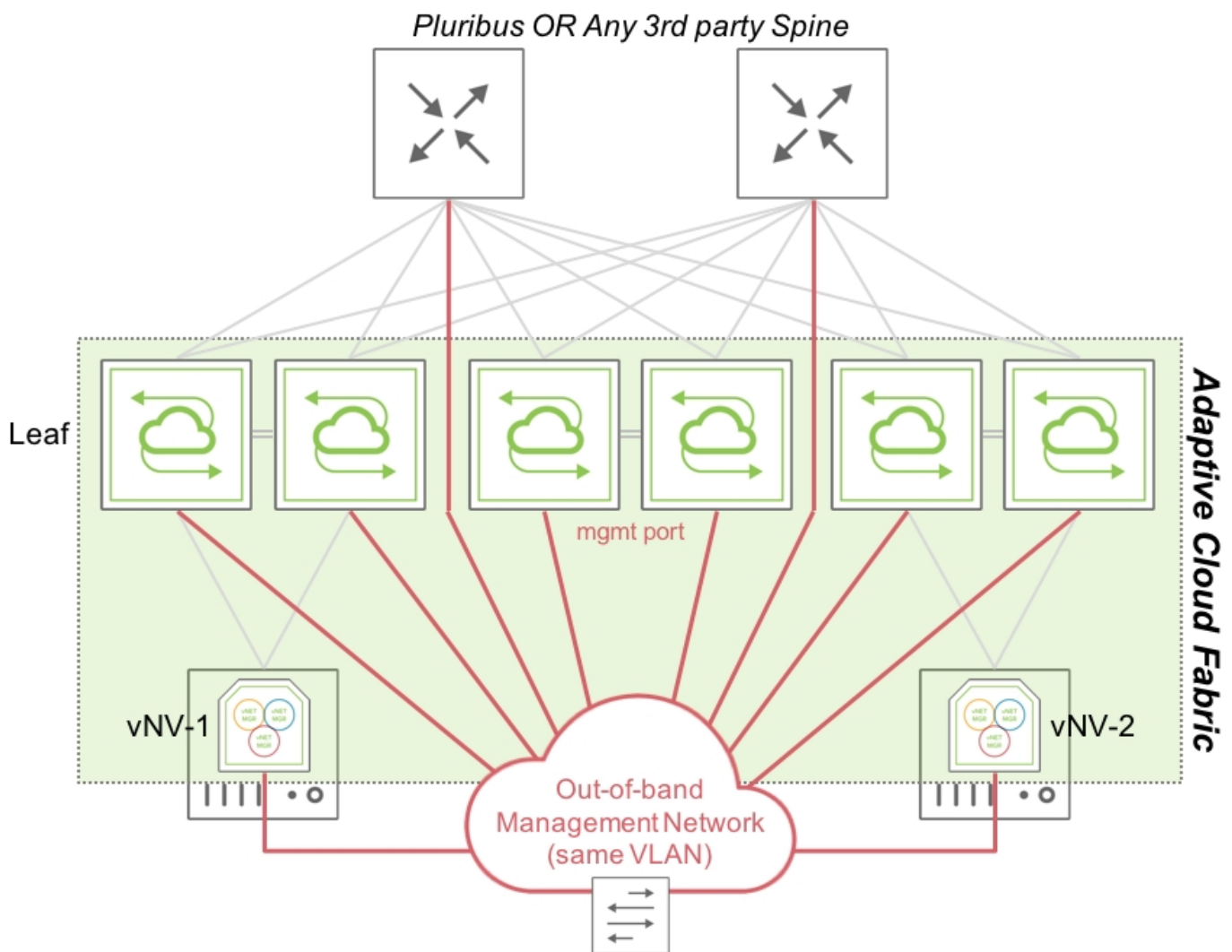
Figure 4 - Fabric Nodes in a "Flat" Management Network
