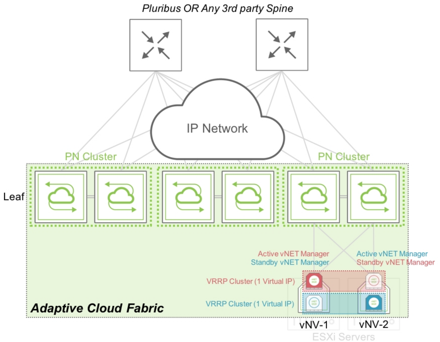
Figure 10 - vNET Manager Redundancy – Active/Standby in a Rack
