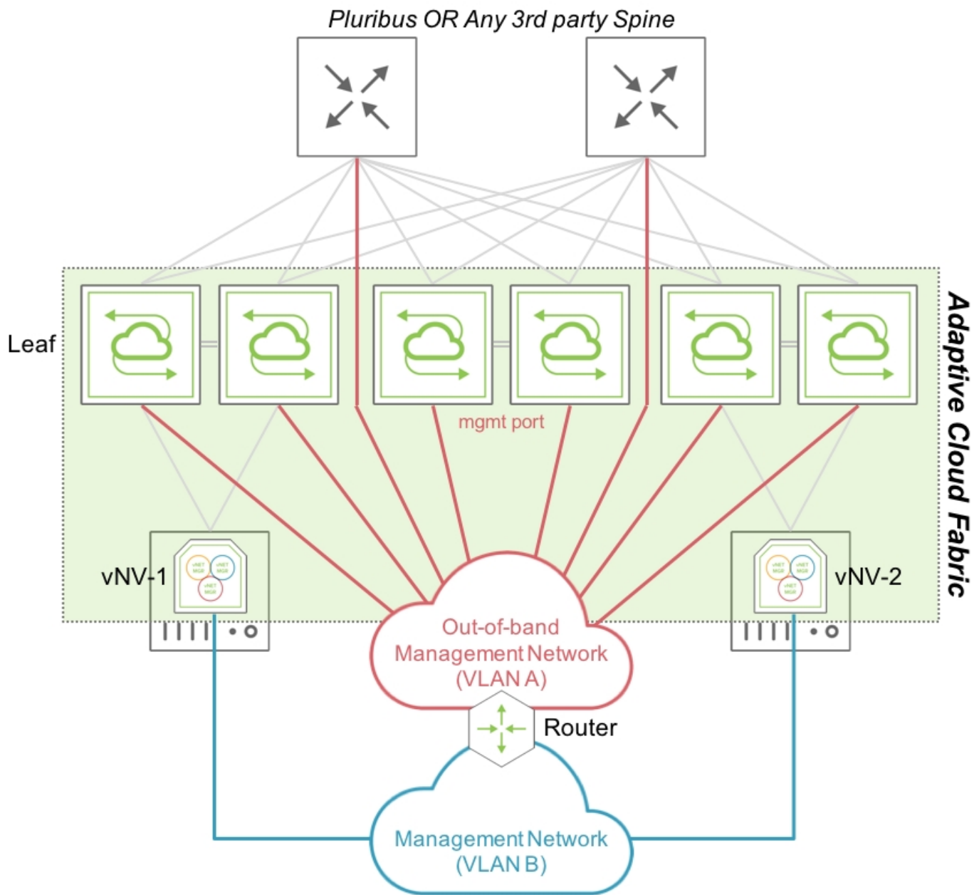
Figure 5 - Fabric Nodes in a Routed Management Network
