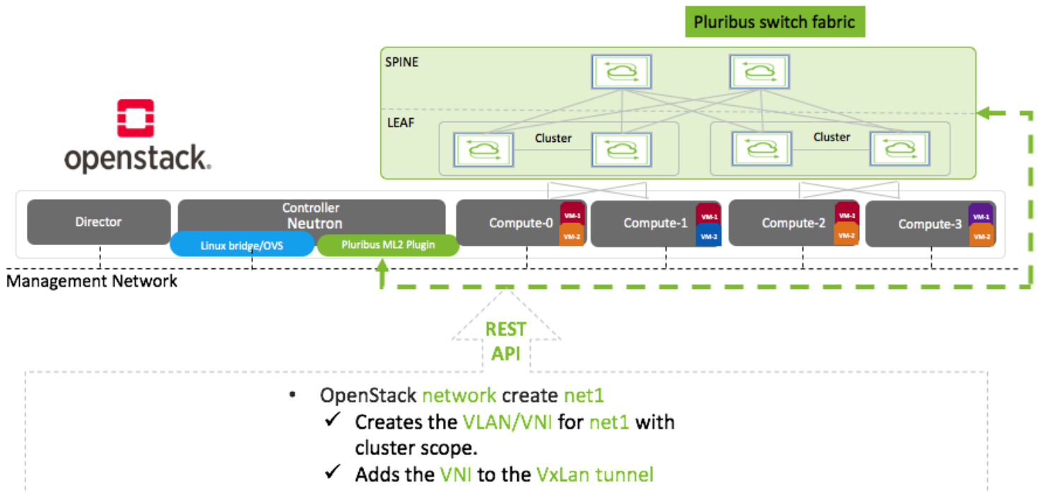
Figure 3: Integration of Unified Cloud Fabric with OpenStack Components using Pluribus ML2 Plugin
