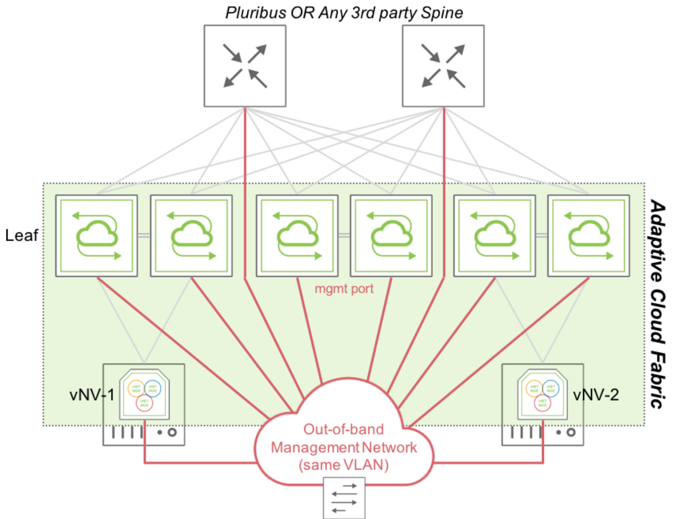
Fabric Nodes in a 'Flat' Management Network
