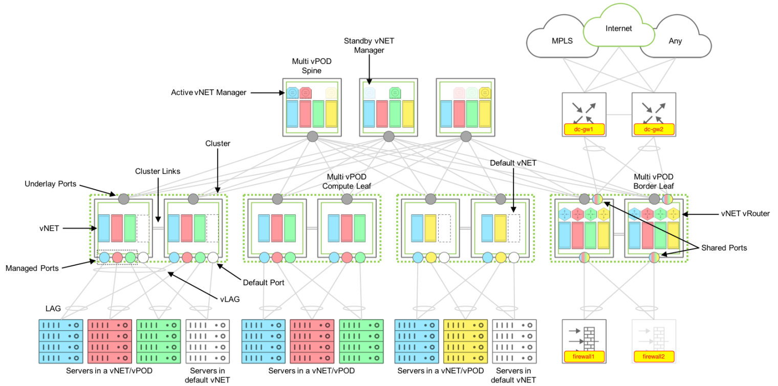
Multitenant Fabric Design Components
