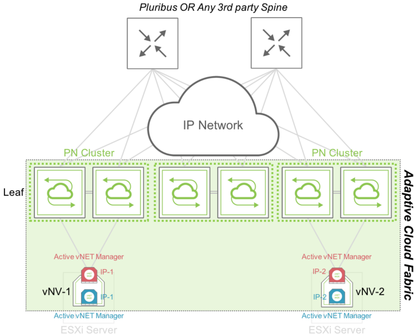
vNET Manager Redundancy – Active/Active between Racks or Datacenters
